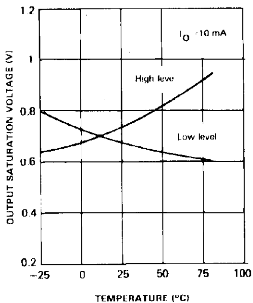
Figure 3: Output Saturation Voltage
